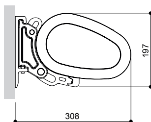
Wandmontage
